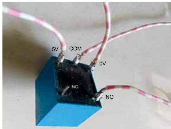
Fig. 4: Pin details of 5V sugar cube relay
